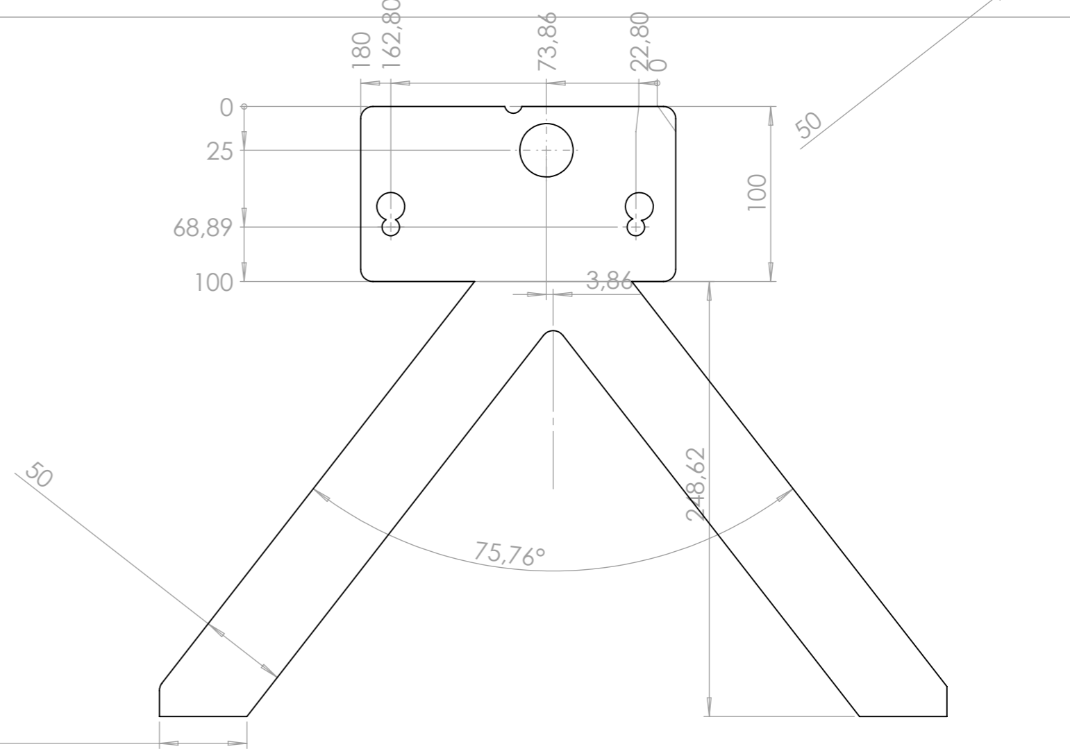
Acier S235
