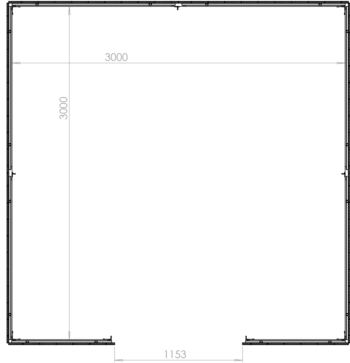
plan B-B
