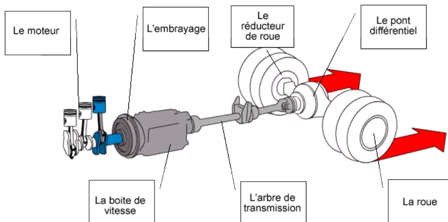
Figure 6: Circuit de transmission mécanique
